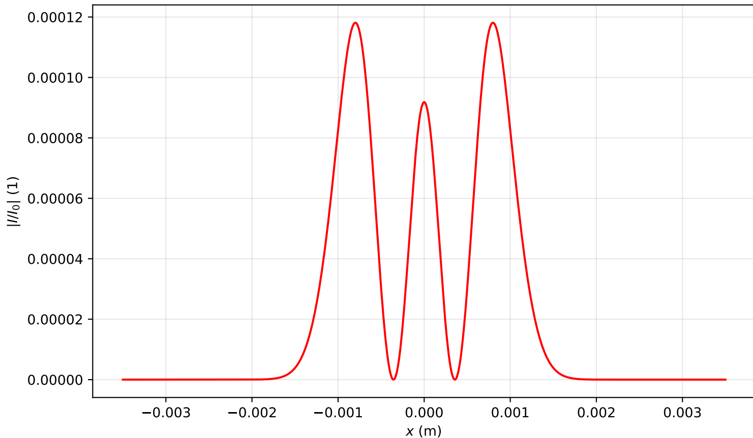
Intensity profile I(x, y = 0, z = 0.398)/I_0 , P_{in}=0.5P_{cr} , artificial time
